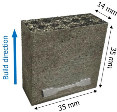
Figure S1 Image of the LPBF block where the tensile direction is added.
