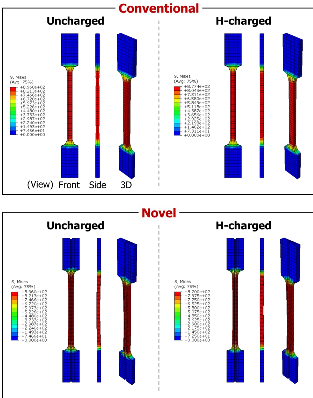
Figure S3 The results from finite element analysis (using ABAQUS 2025) for the von Mises stress distributions in the conventional and novel tensile specimens in uncharged and H-charged states.
