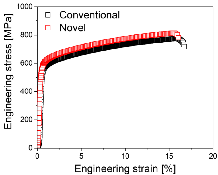
Figure S2 Representative engineering stress-engineering strain curves obtained from tensile tests using conventional and novel geometry specimens.
