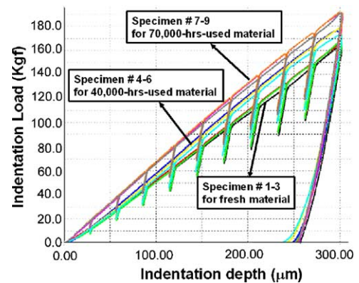
Fig. 2. Superposition of load–displacement curves obtained from multiple indentations of Cr–Ni steels.
