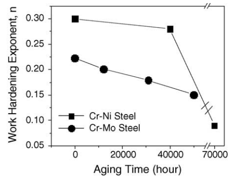
Fig. 5. Change in work-hardening exponent with aging time (at room temperature).
