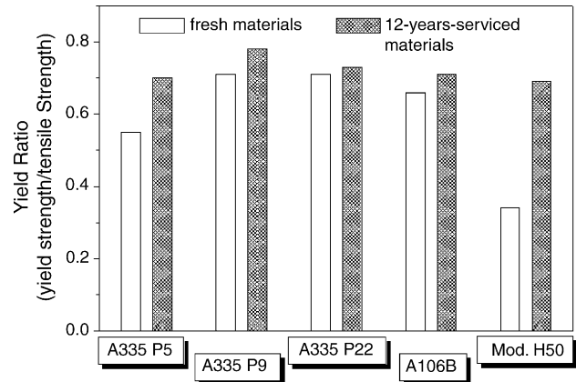
Fig. 7. Comparison of yield ratio between new materials and 12-year-served materials.
