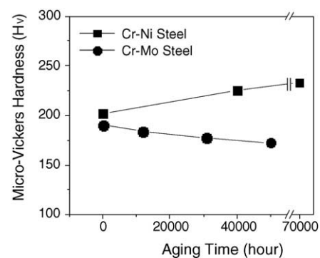
Fig. 3. Change in micro-Vickers hardness with aging time (at room temperature).
