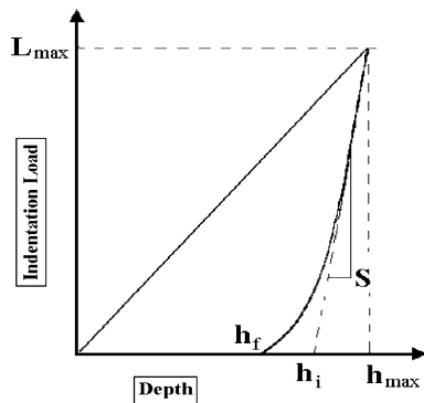
Fig. 1. Schematic diagram of typical load–depth curve obtainable during instrumented spherical indentations on steel.
