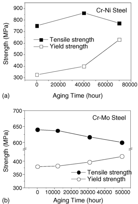
Fig. 4. Variations in tensile and yield strength with increasing aging time (at room temperature): (a) Cr–Ni steel and (b) Cr–Mo steel.
