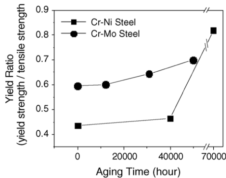
Fig. 6. Change in yield ratio with increasing aging time.
