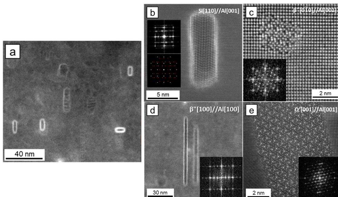
Fig. 8. (a) Overview image of HAADF-STEM and (b-e) magnified images representing the nanostructure of the precipitates in MT820. All TEM images were obtained along the [100]_{\text{Al}} zone axis.
