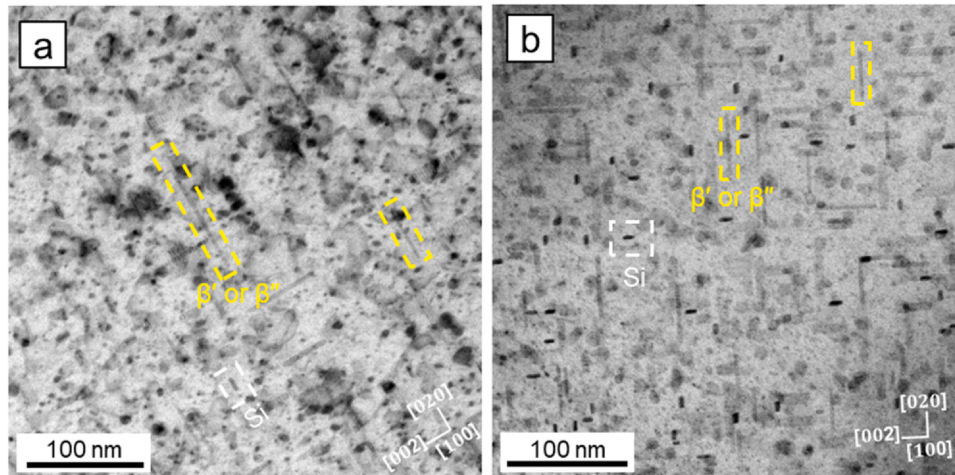
Fig. 7. TEM micrographs of (a) MT720 and (b) MT820 obtained along the [100]_{\text{Al}} zone axis.
